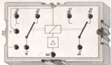
1 Relais-Baustein
